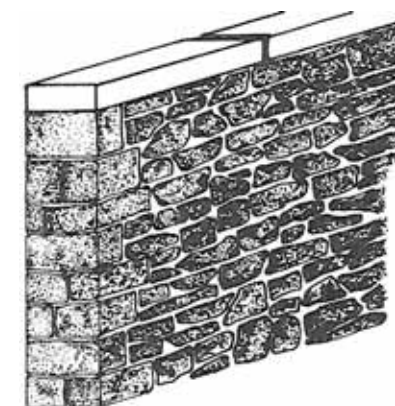
Traditional random rubble stone wall with flat stone coping.
