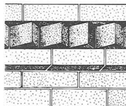
Below: Projecting decorative brickwork - typical South Derbyshire eaves details.
